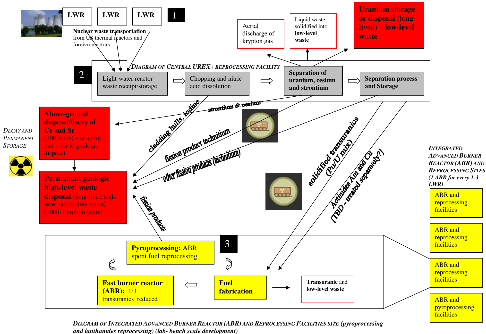
Graph representing Department of Energy/Argonne National Laboratories proposal for reprocessing and transmuting nuclear waste as part of the Global Nuclear Energy Partnership (2007 iteration)
